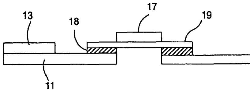
(RELATED ART) FIG. 1
